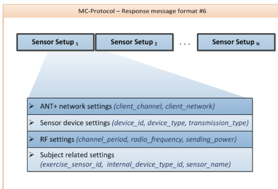
Figure 4. Response message format #6.
