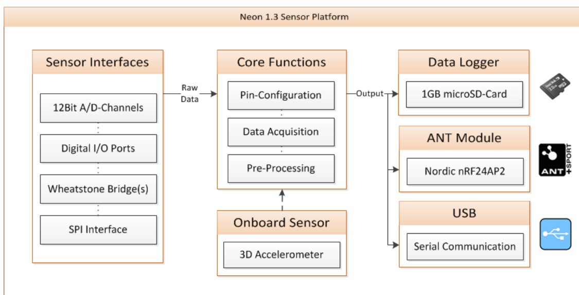
Figure 2. Systematic overview of the used sensor platform.
