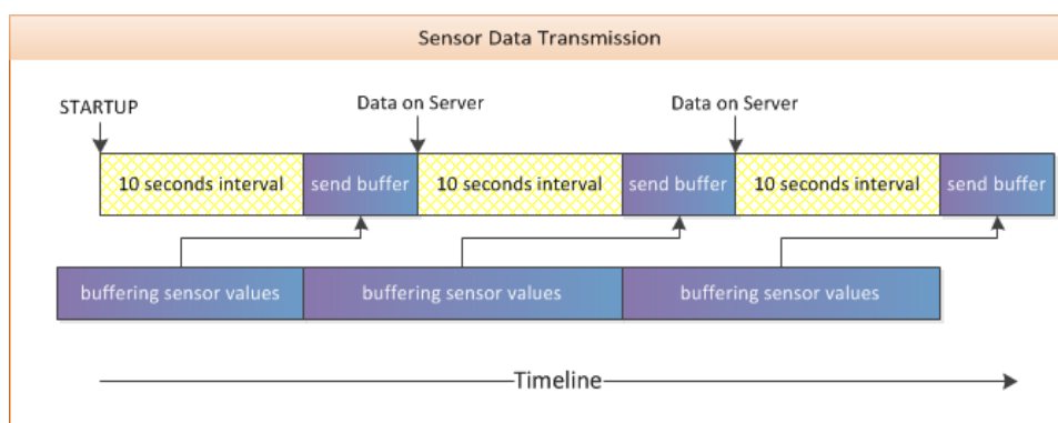
Figure 7. Sensor data transmission timing.
