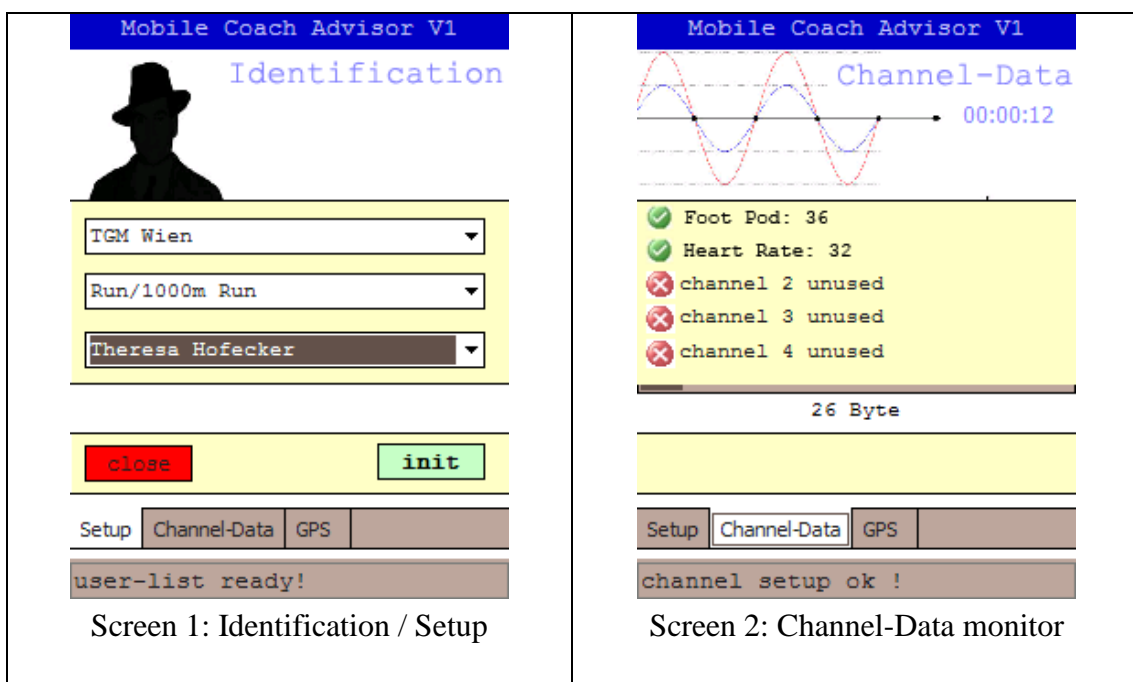
Figure 6. GUI of the A-Client application.
