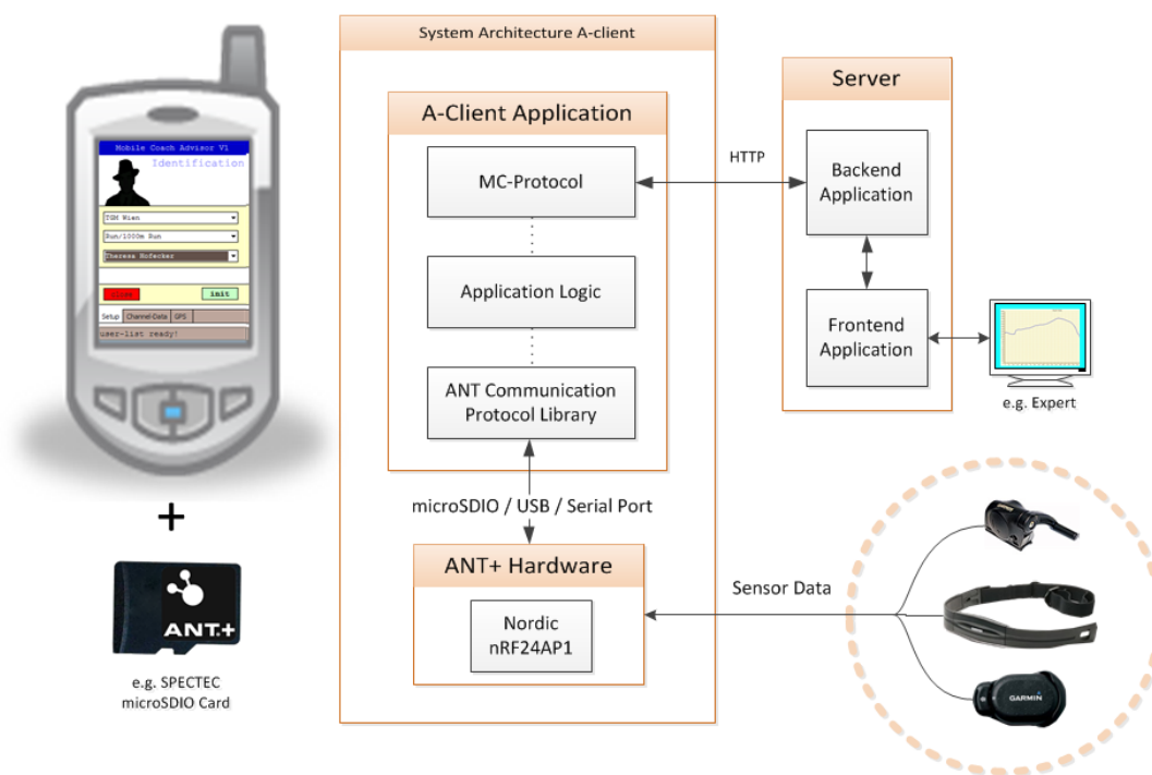
Figure 3. Architecture of the A-Client.
