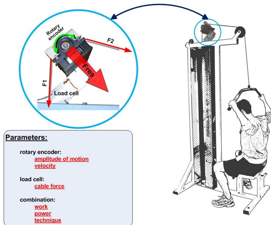
Figure 11. Implementation of a load cell and a rotary encoder into an exercising machine.
